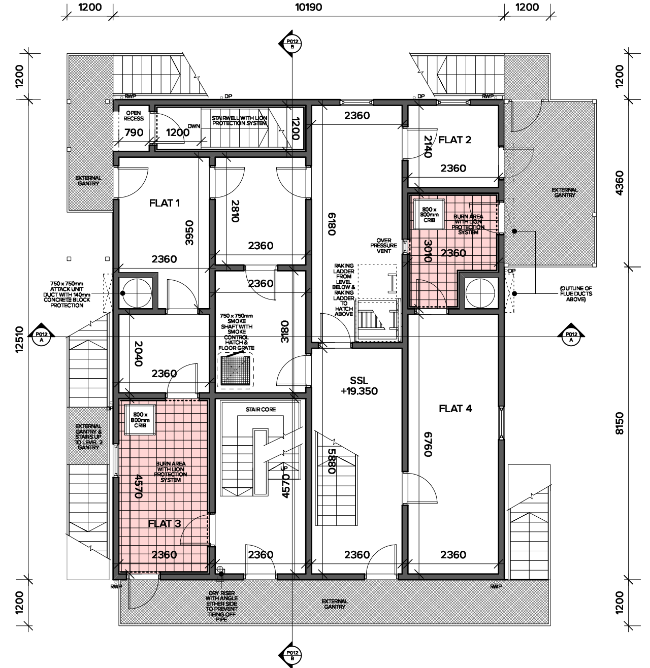
PROPOSED FIRST FLOOR PLAN SSL +19.350
