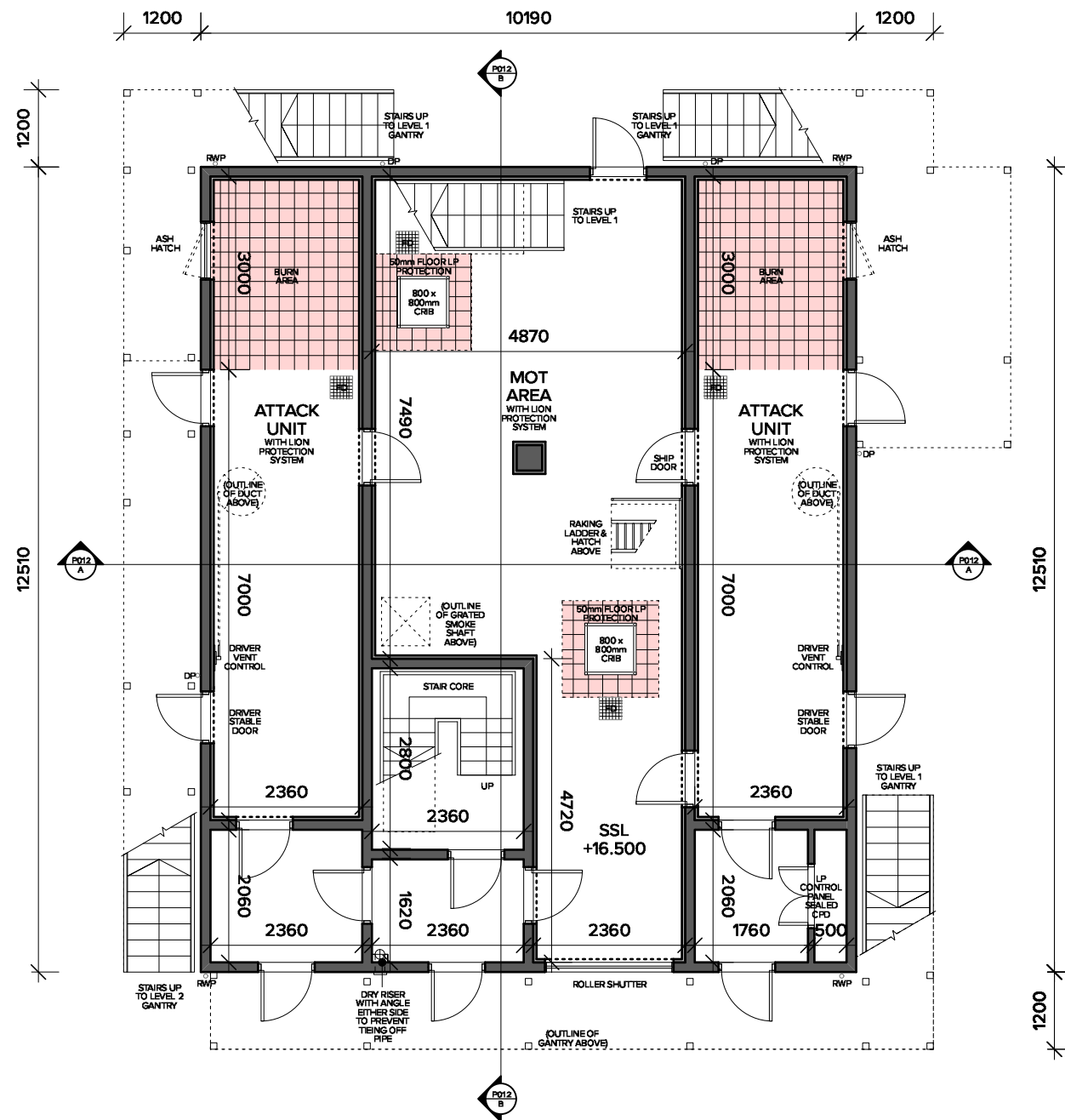
PROPOSED GROUND FLOOR PLAN SSL +16.500
