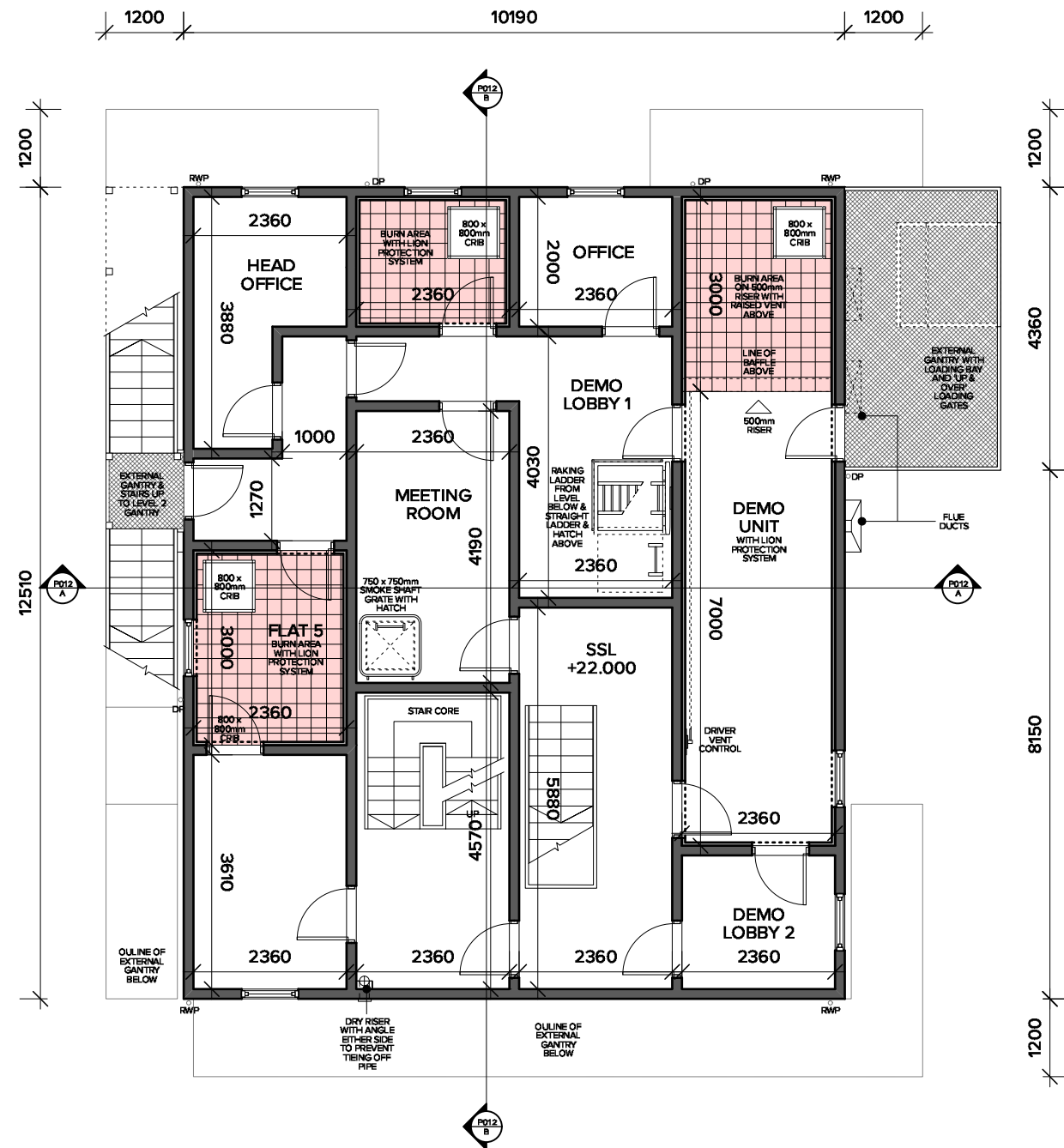
PROPOSED SECOND FLOOR PLAN SSL +22.000
