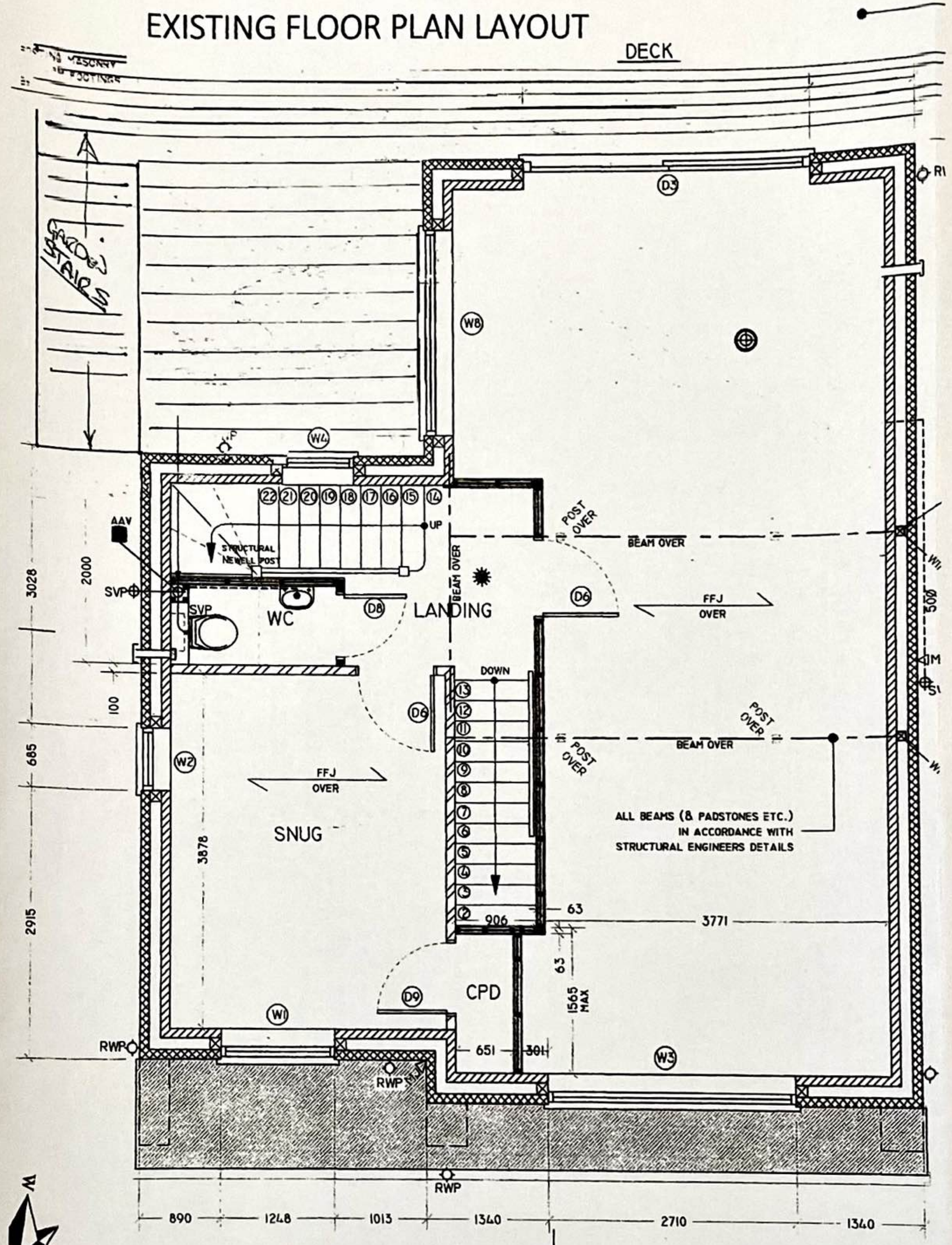
EXISTING GROUND FLOOR \triangle FRONT \triangle
