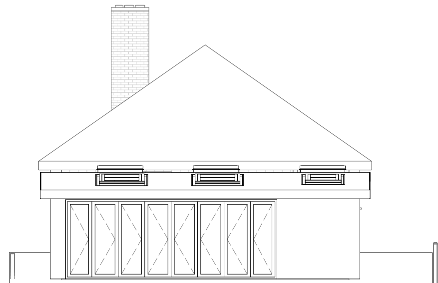
Proposed Elevation-Rear
