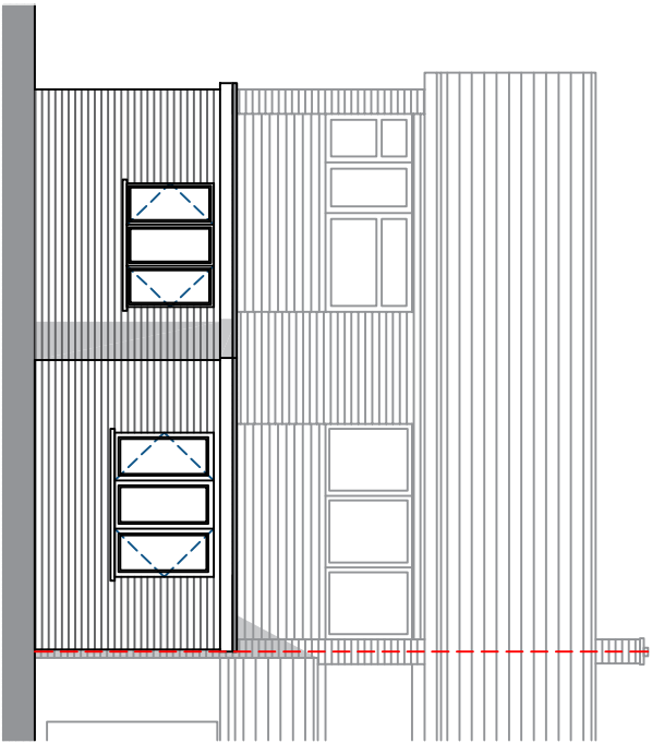
Proposed Rear Elevation 1:100 @ A3
