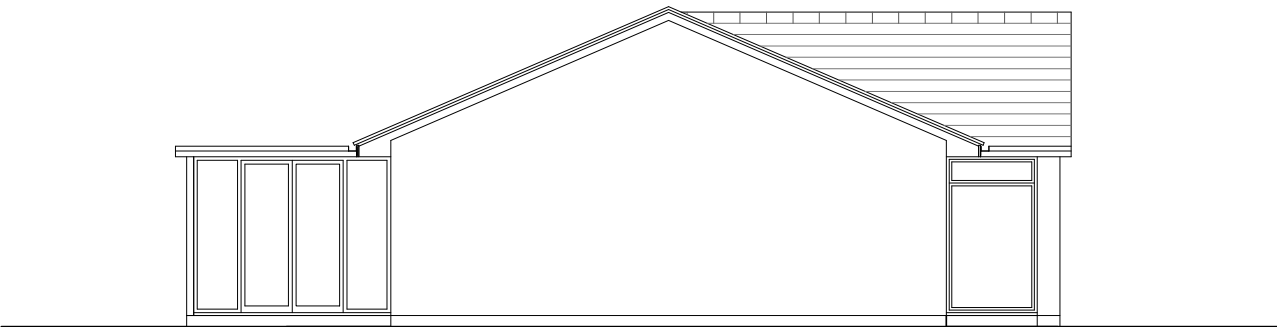
WEST ELEVATION
