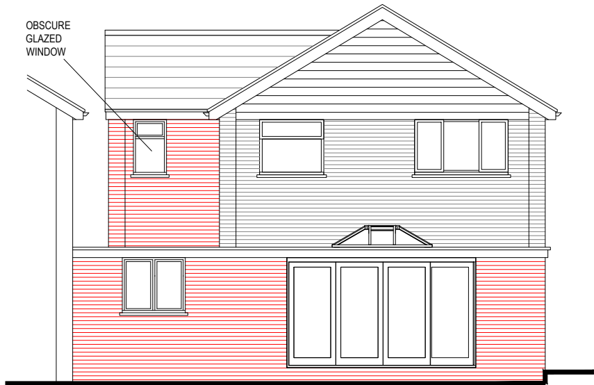
REAR ELEVATION
