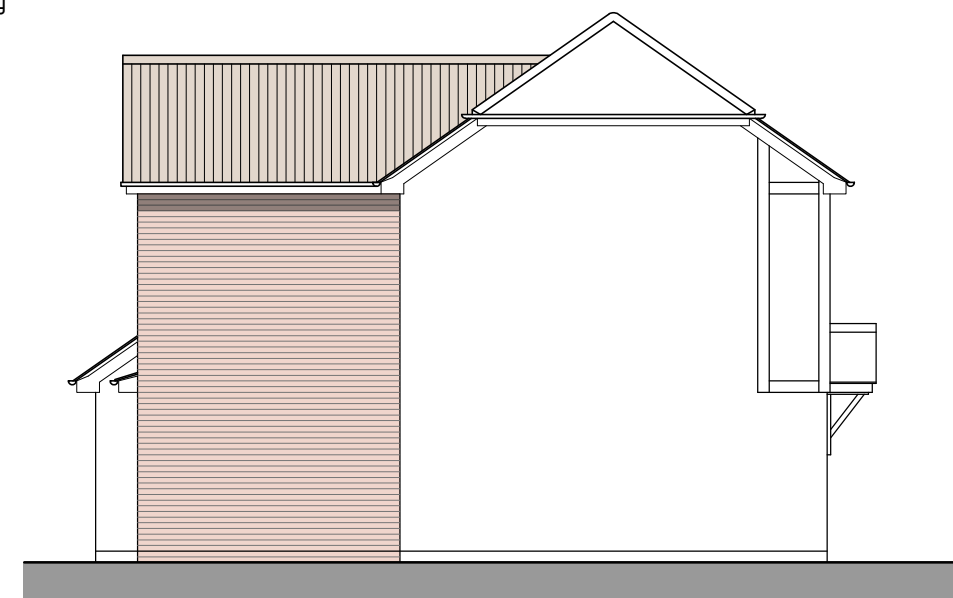
SIDE ELEVATION
