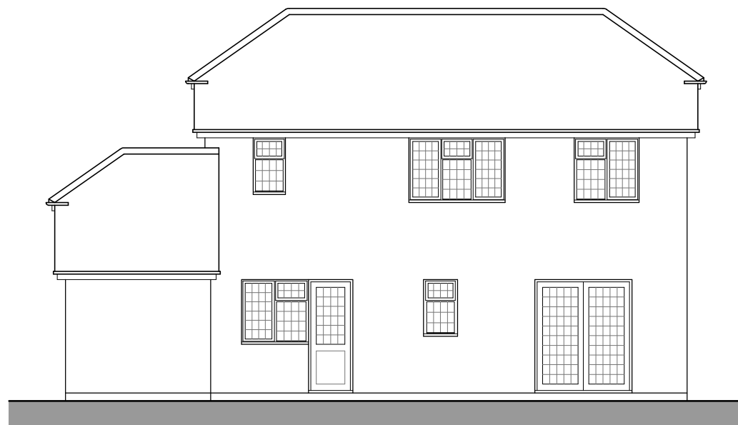
REAR ELEVATION
