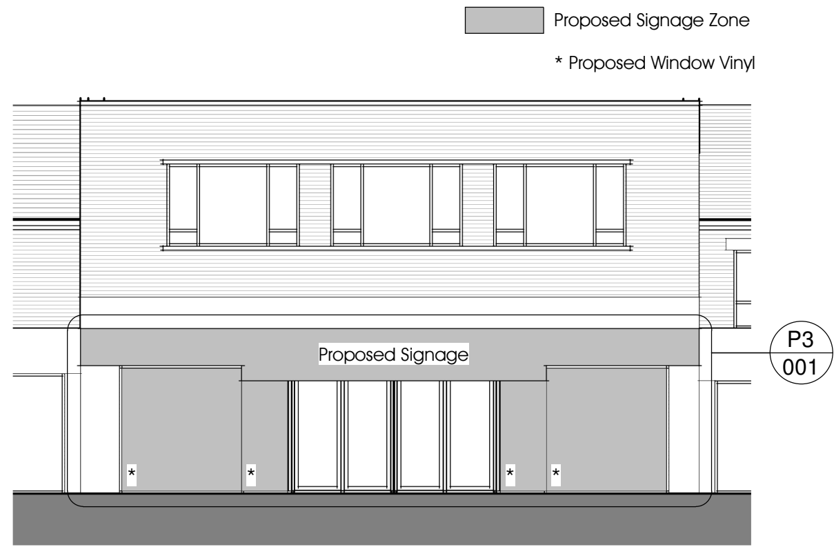
P1 Proposed Front Elevation 1 : 100
