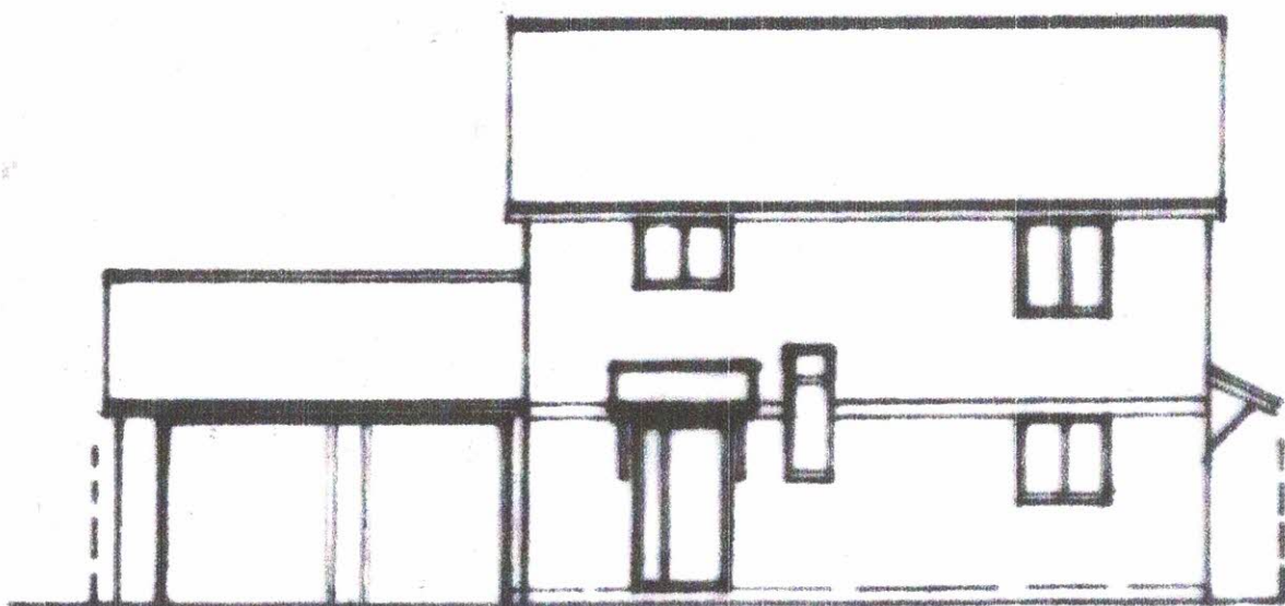
FRONT (WEST)
