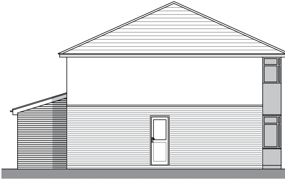
Proposed Side Elevation 1:100 @ A3
