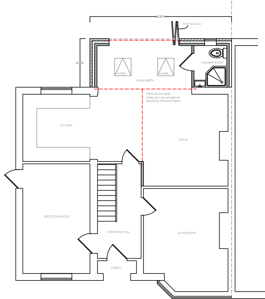
Proposed Ground Floor Plan 1:100 @ A3
