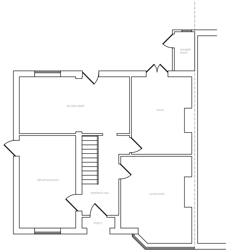
Existing Ground Floor Plan 1:100 @ A3
