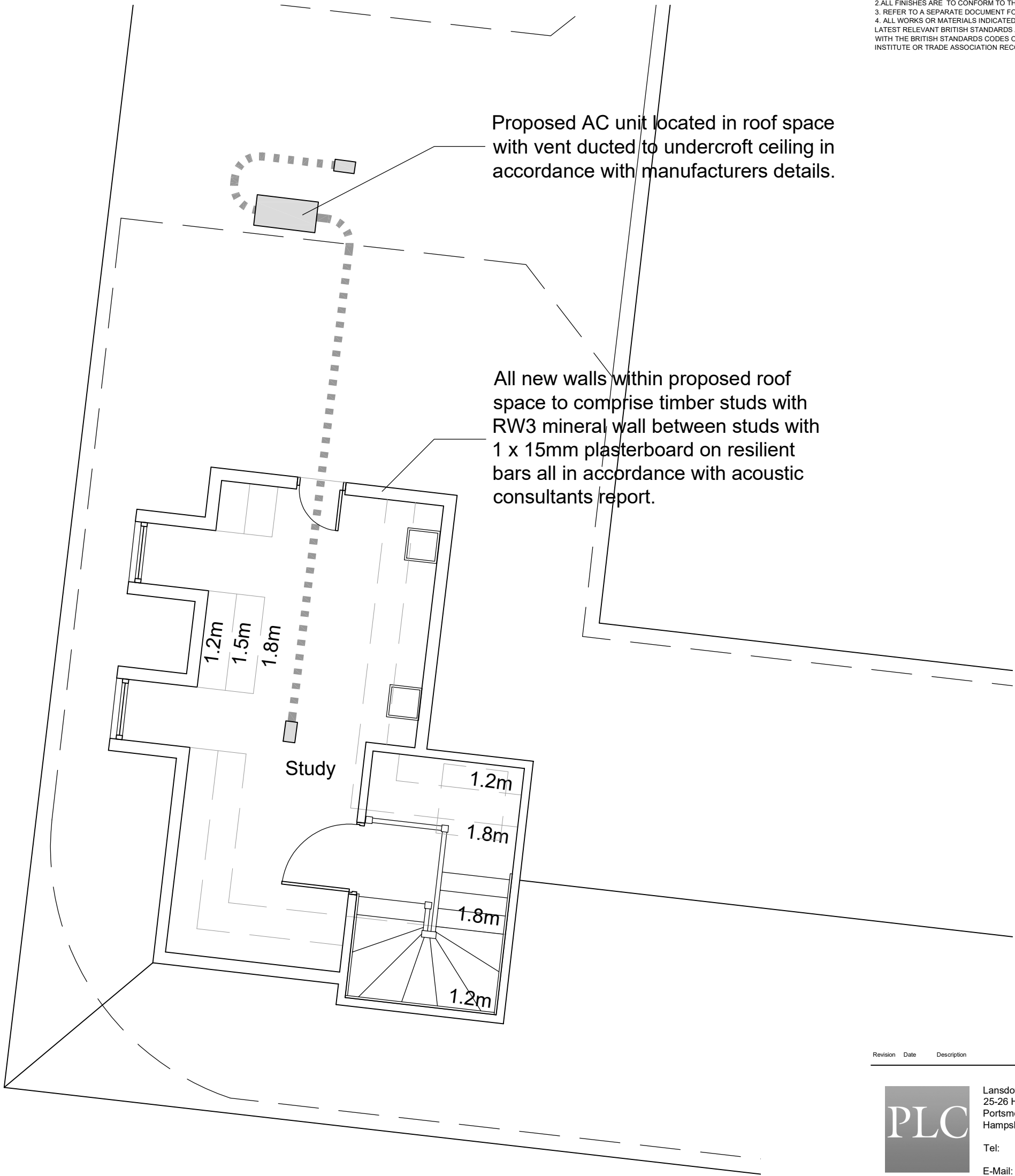
FIRST FLOOR / ROOF PLAN
