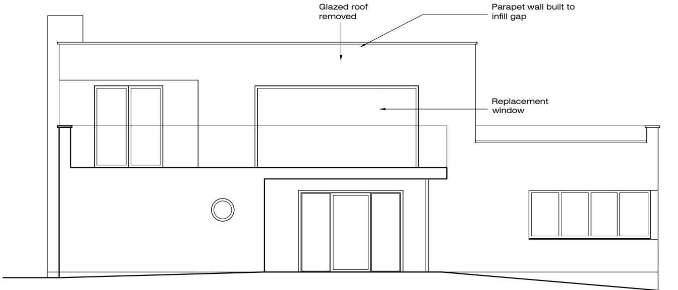
East Elevation - As Proposed
