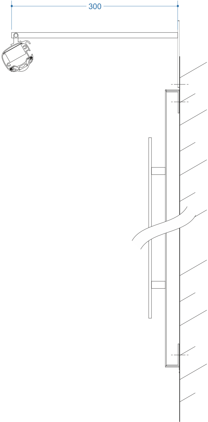
Sectional Detail Scale: 1:4 @A3
