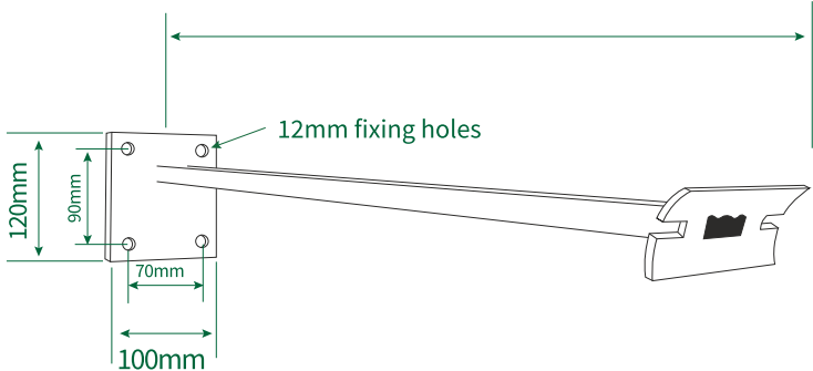
Trough Light Bracket Detail
