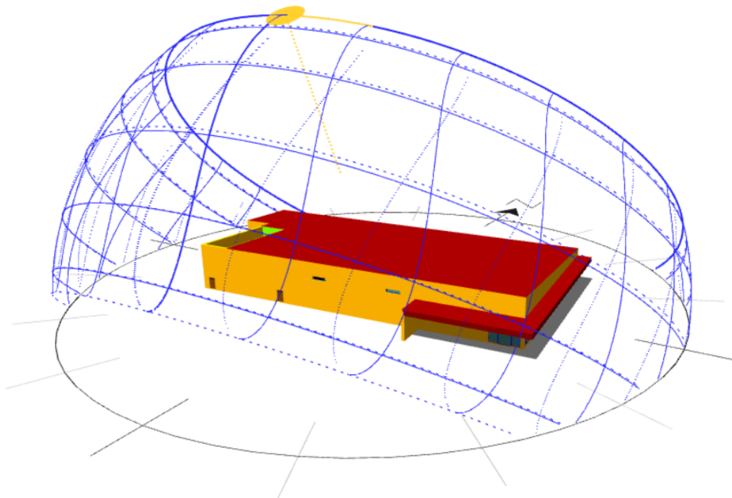
Figure 9 - Orientation & Sun Path Image
