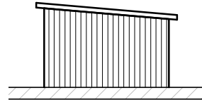
4 Bike store side 1 : 100
