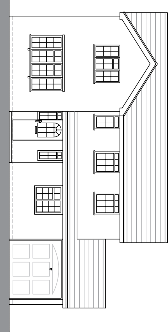
Existing Front Elevation | : 100 @ A3
