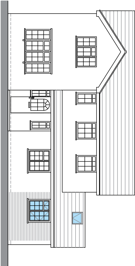
Proposed Front Elevation | : 100 @ A3
