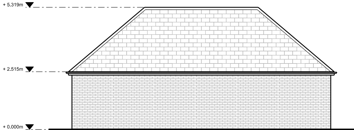
Rear Elevation
