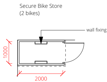
Floor Plan
