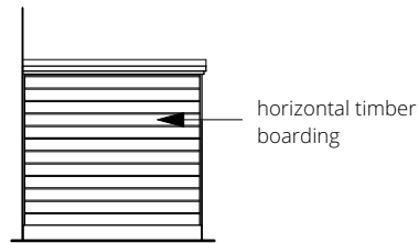
East Elevation
