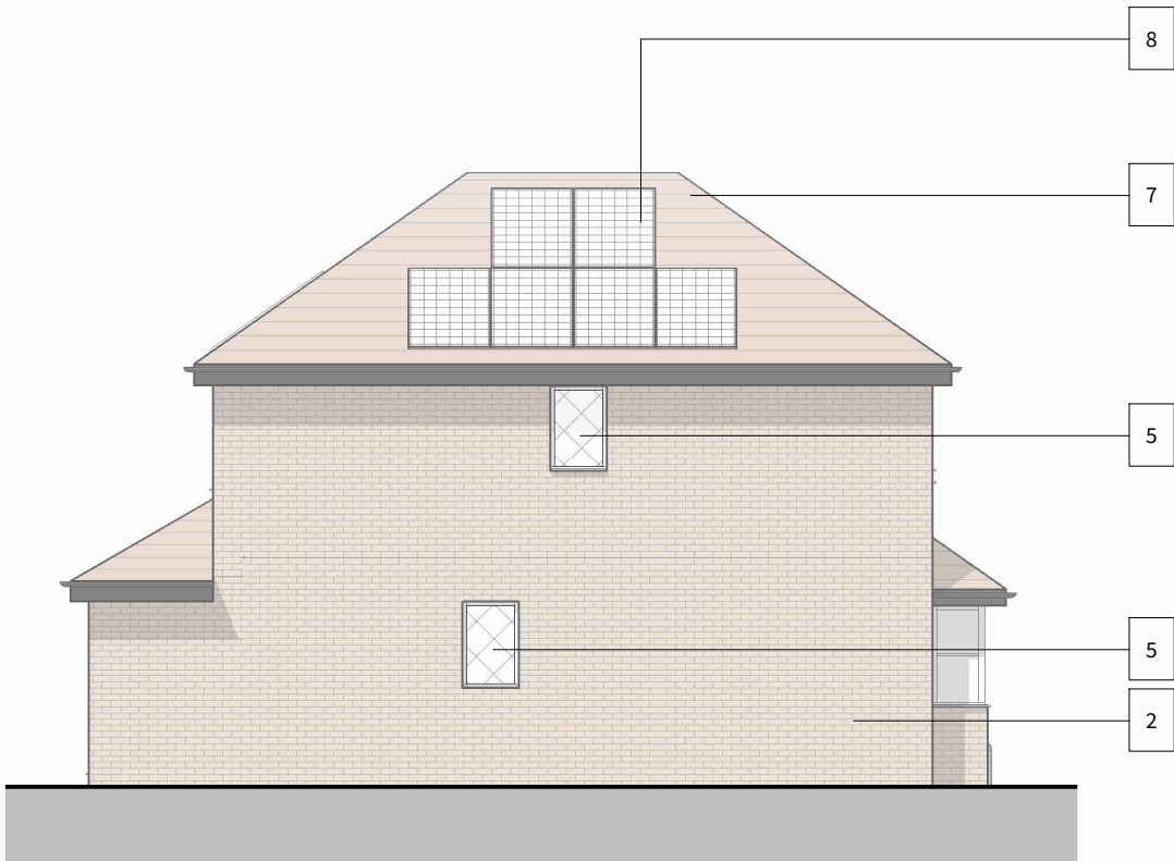
2 North West Elevation - 1 : 100
