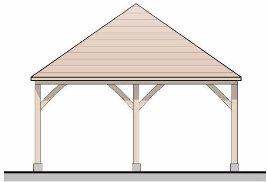
1 Front Elevation - 1 : 100
