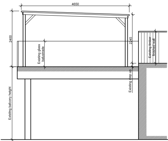
Section through SCALE 1:100
