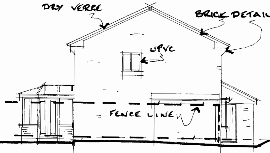
South Elevation
