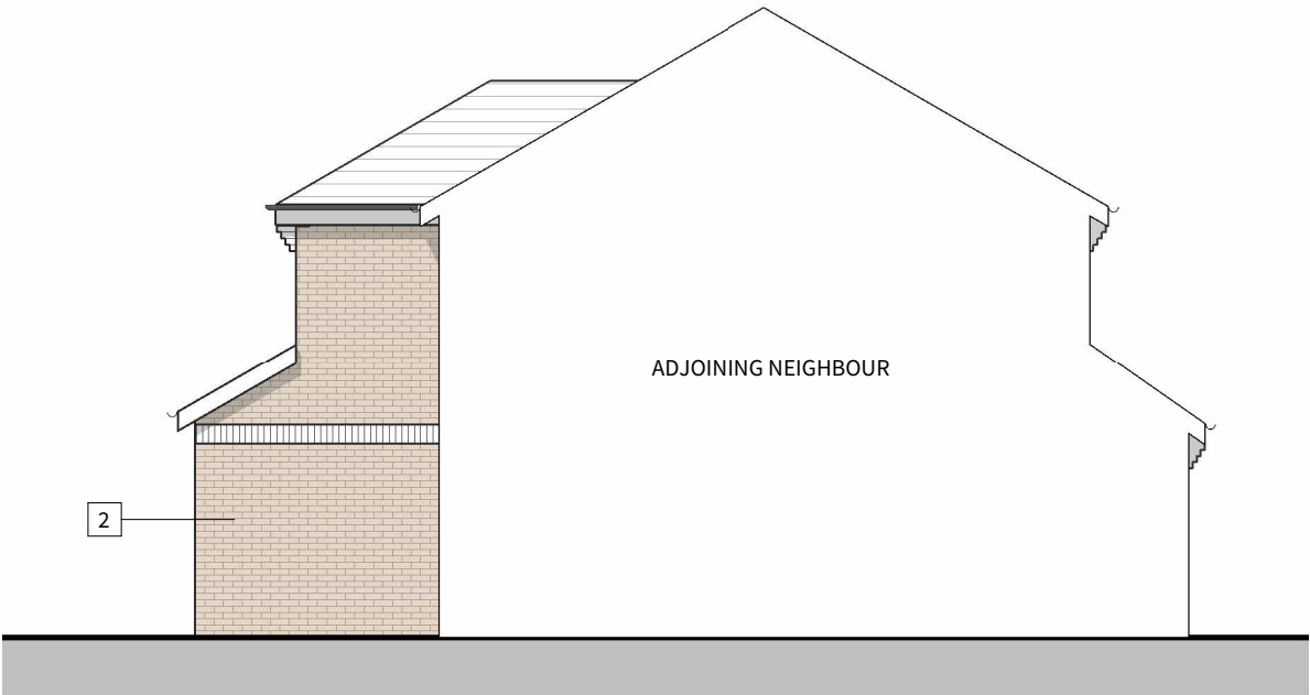
2 East Elevation - 1 : 100
