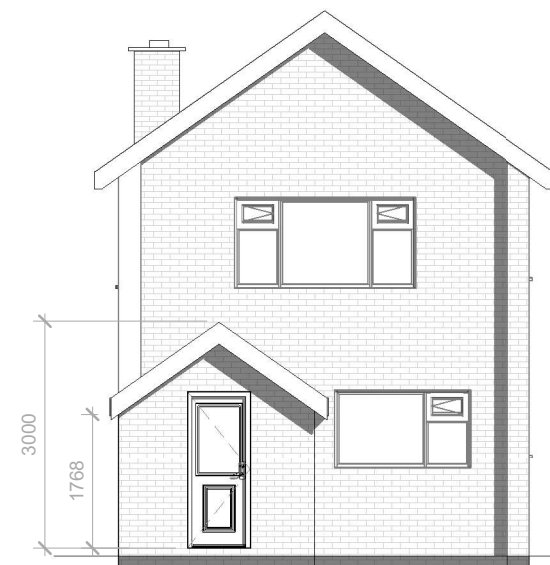
Proposed Elevation-Front
