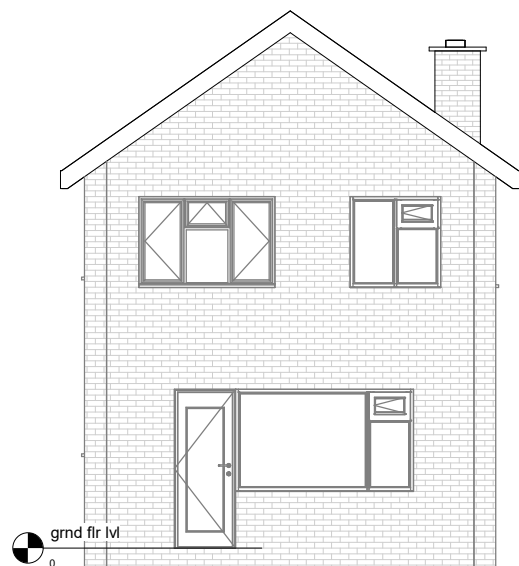
Existing Elevation-Rear
