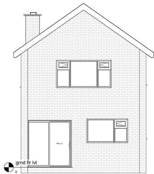
Existing Elevation-Front
