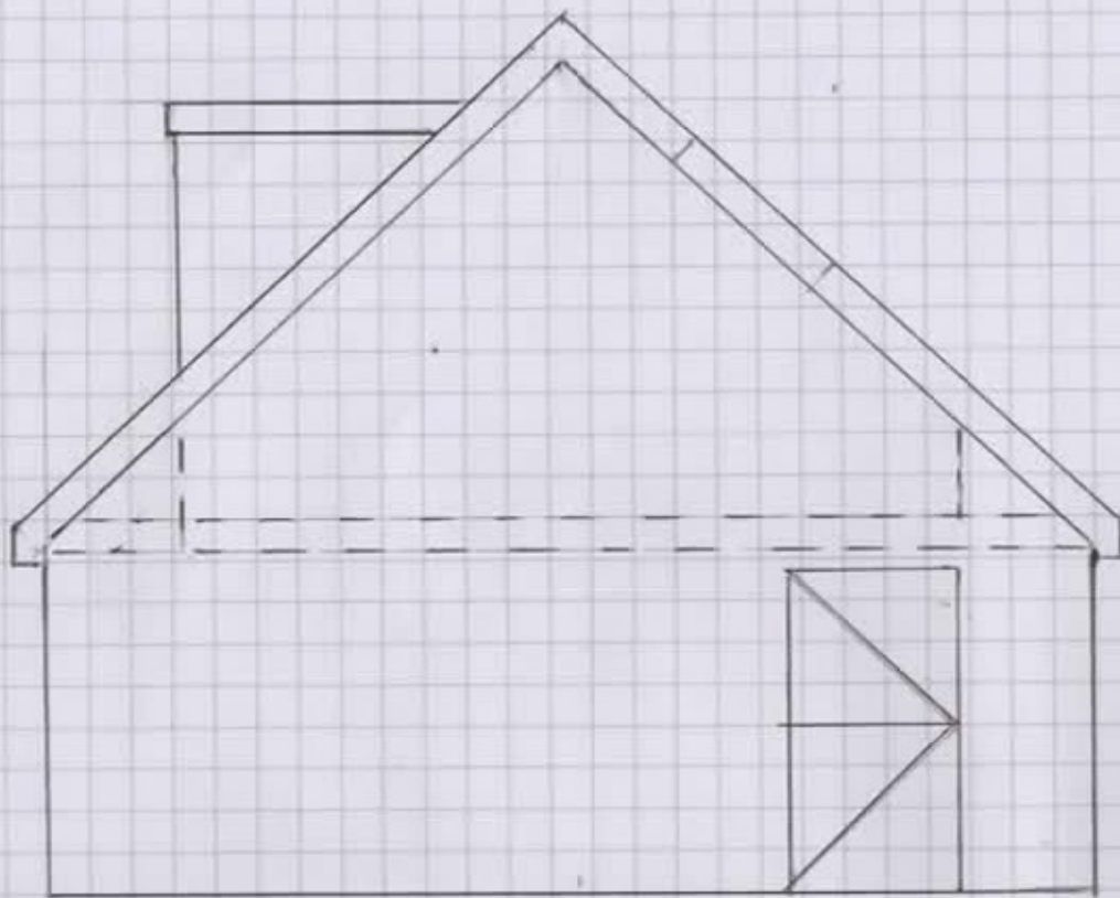
NORTH FACING SIDE PROPOSED SCALE 1:50 AT A4
