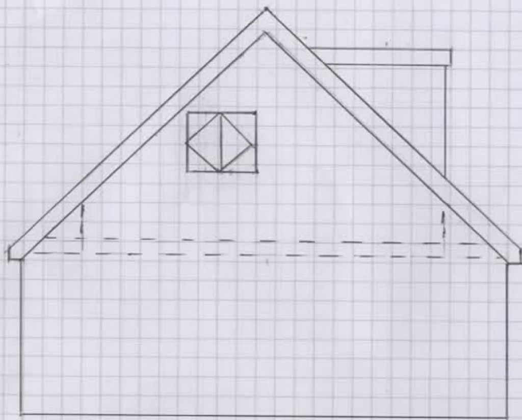
SOUTH FACING SIDE PROPOSED SCALE 1:50 AT A4
