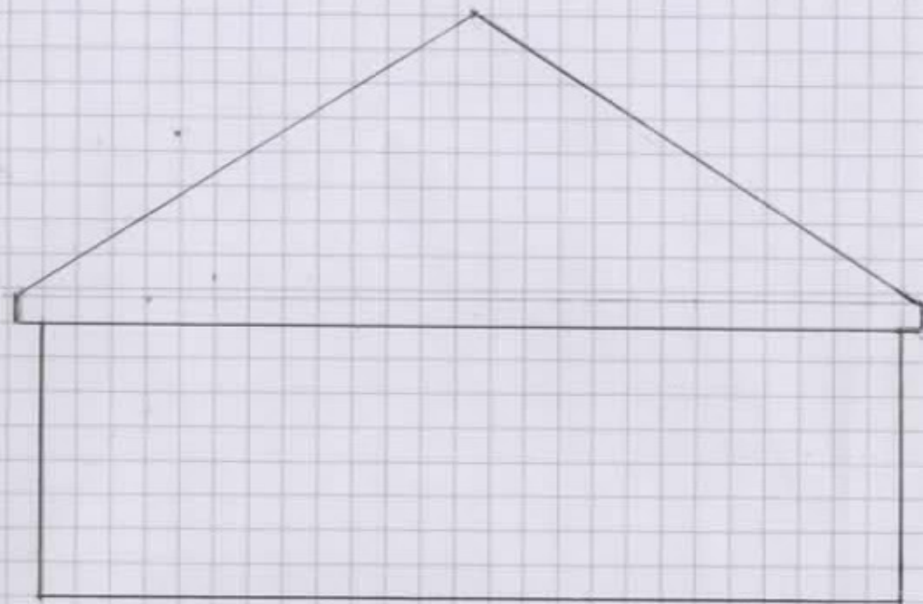
SOUTH FACING SIDE EXISTING SCALE 1:50 AT A4
