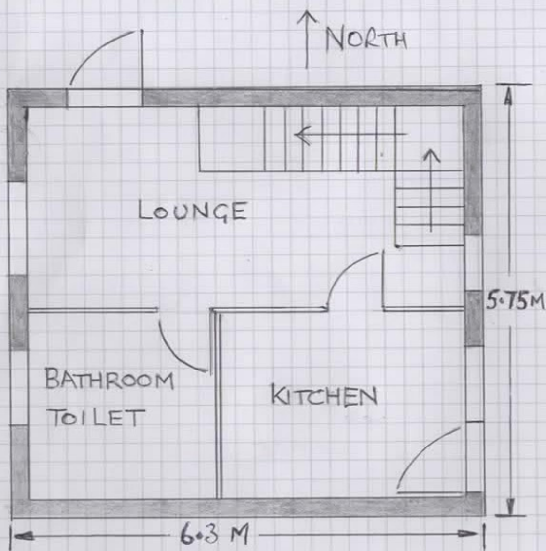
PROPOSED PLAN GROUND FLOOR SCALE 1:50 AT A4
