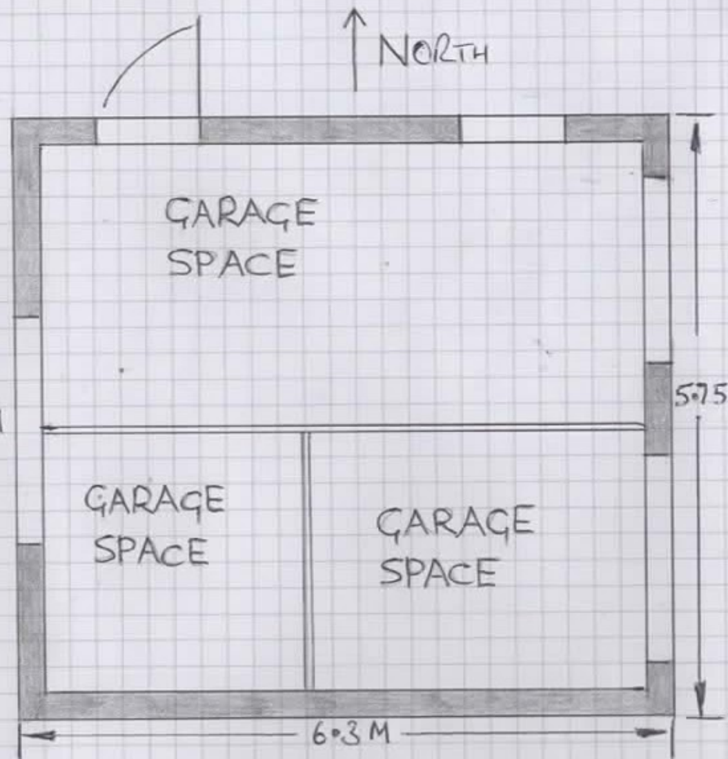
EXISTING PLAN GROUND FLOOR SCALE 1:50 AT A4
