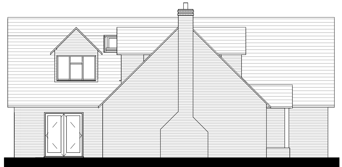
Proposed Side 1 1 : 100
