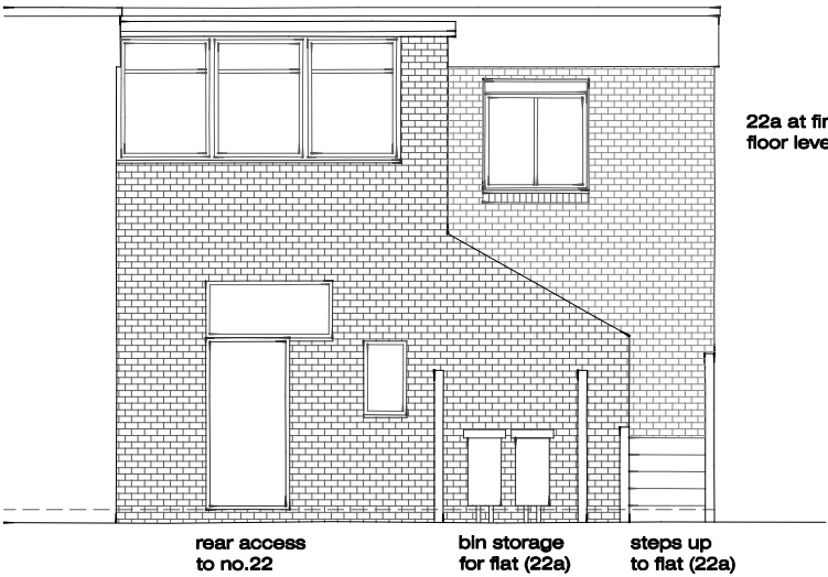
North-West (Rear) Elevation - As Existing
