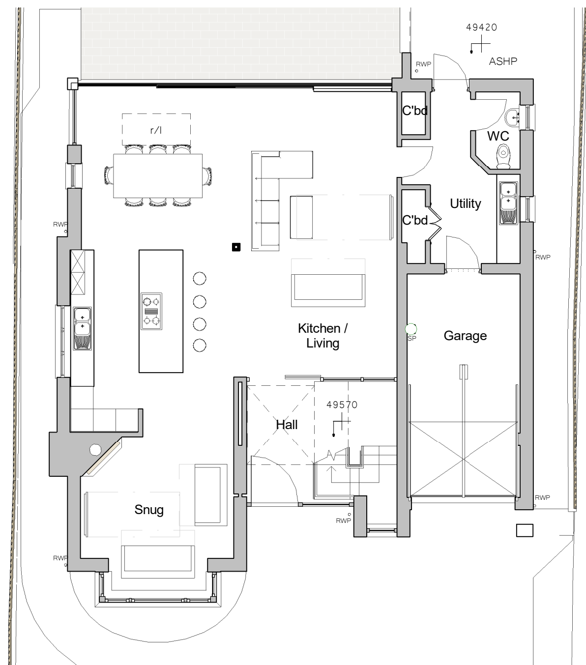
Ground Floor Plan as Proposed 1 : 100
