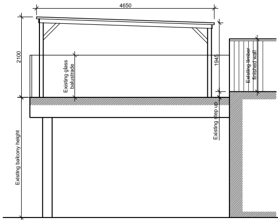
Section through SCALE 1:100
