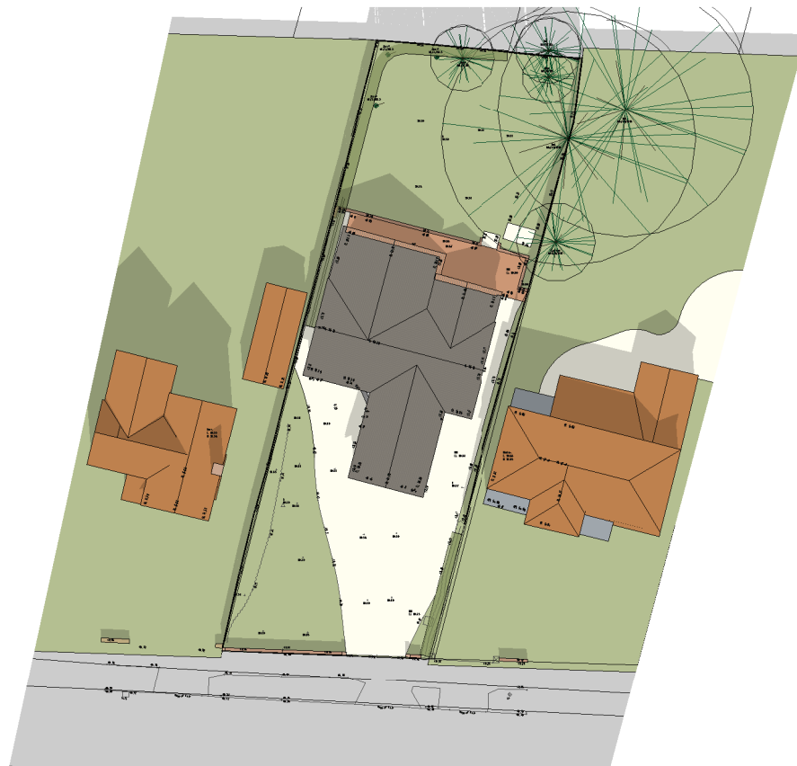
2 Existing - Spring Equinox 1200 1 : 500
