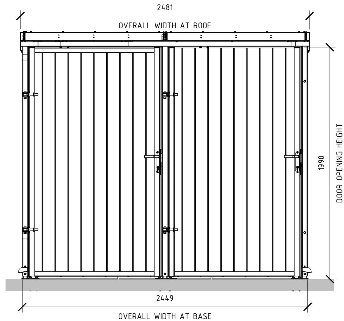
Front Elevation 1 : 20
