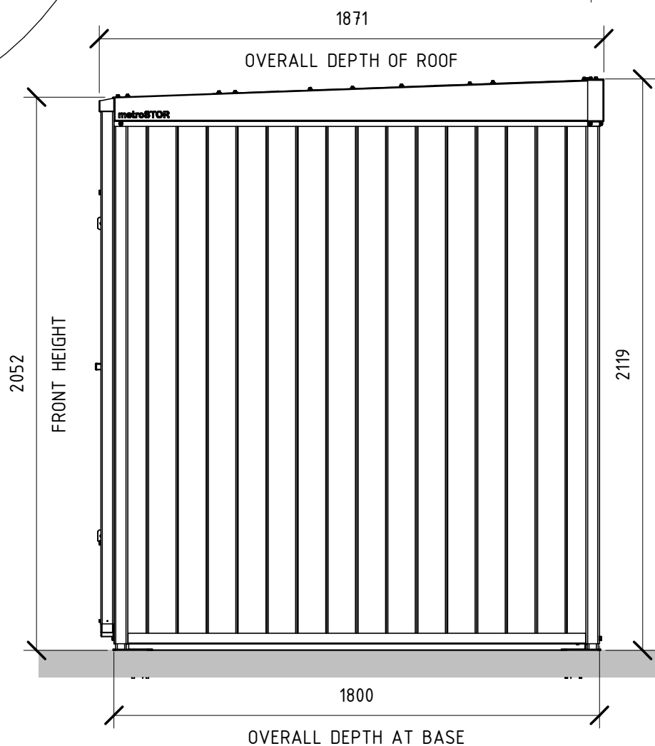
Side Elevation 1 : 20
