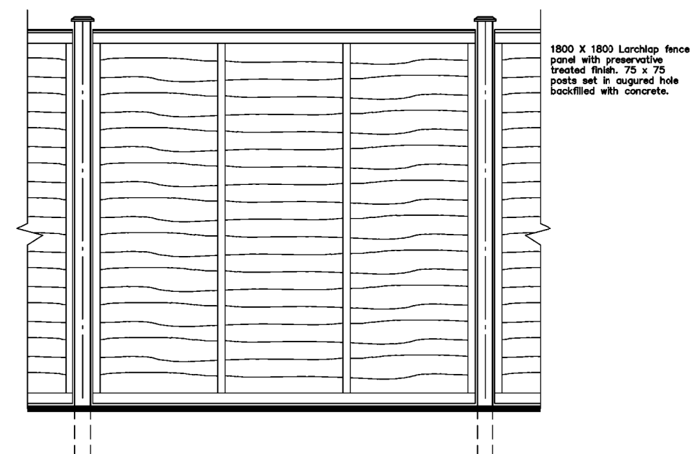
LARCHLAP FENCE
