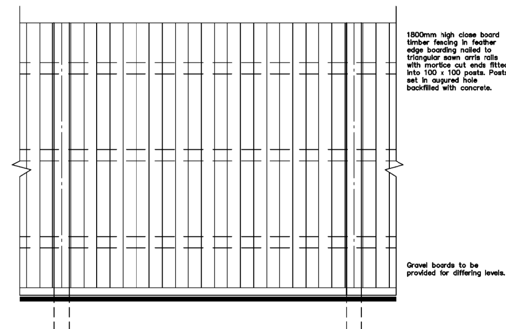
CLOSE BOARDED FENCE
