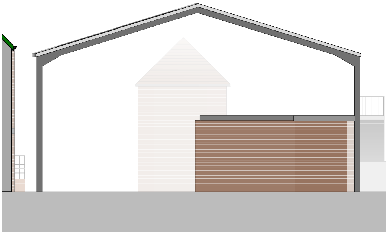
North Elevation existing 1 : 100
