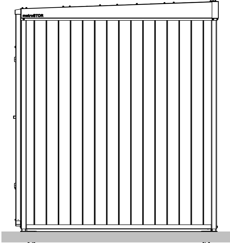
Proposed Side Elevation 1 1 : 20
