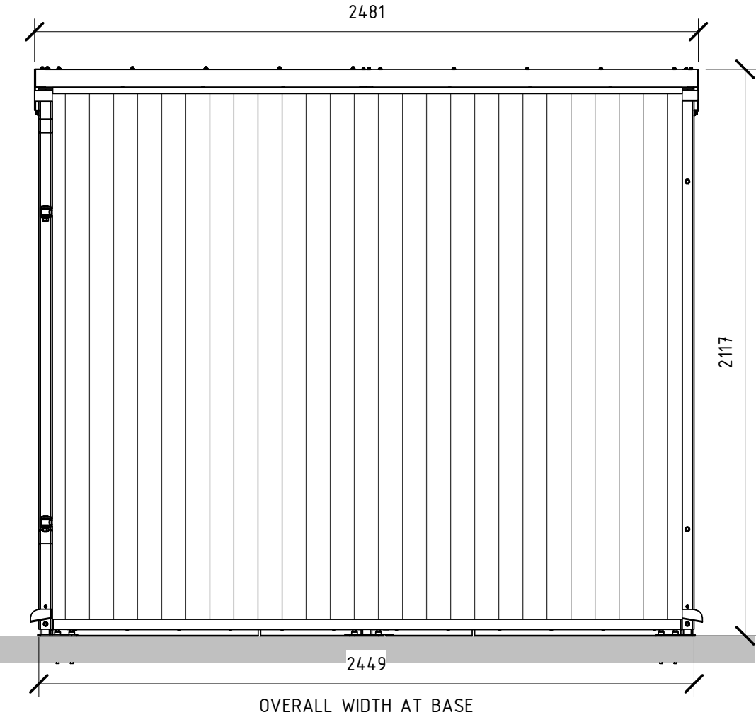
Proposed Back Elevation 1 : 20
