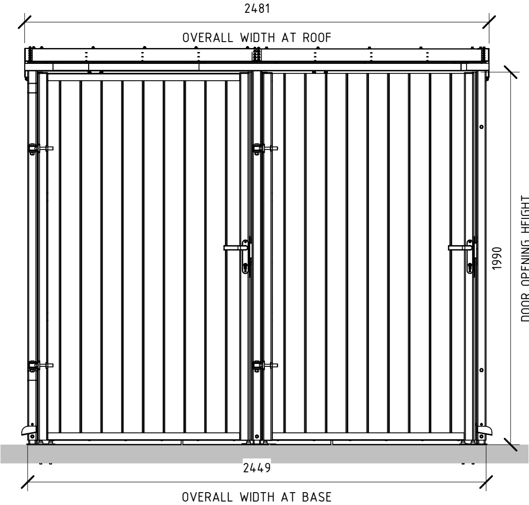
Proposed Front Elevation 1 : 20
