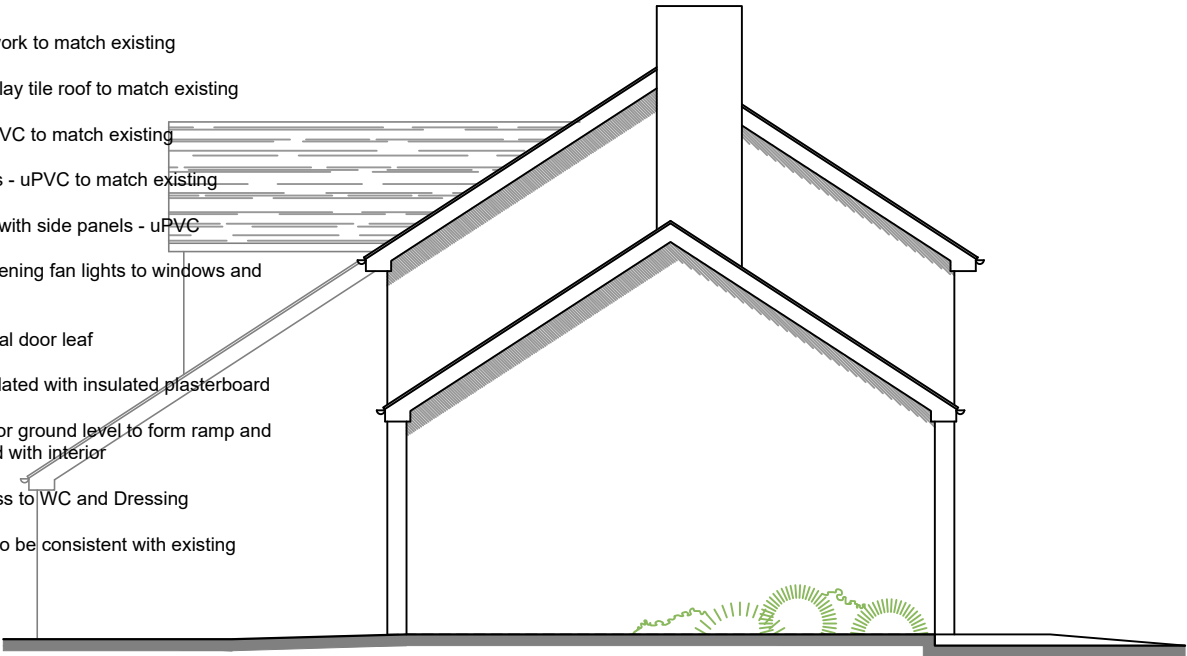
WEST ELEVATION
