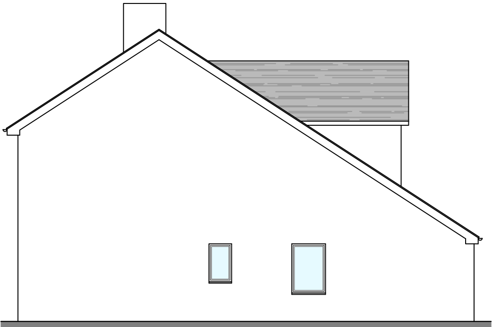
EAST ELEVATION
