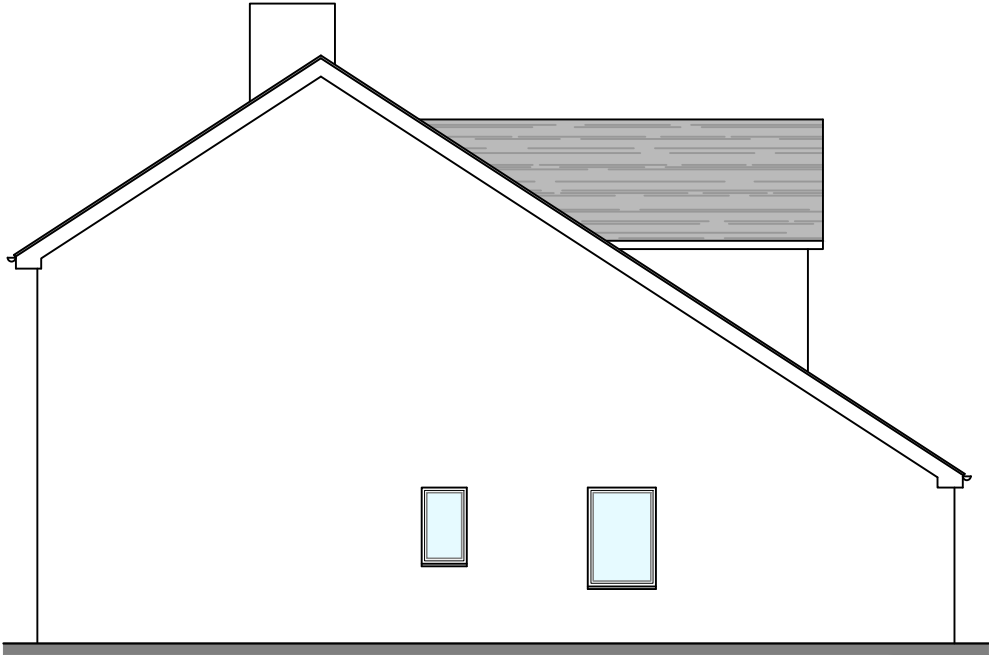
EAST ELEVATION
