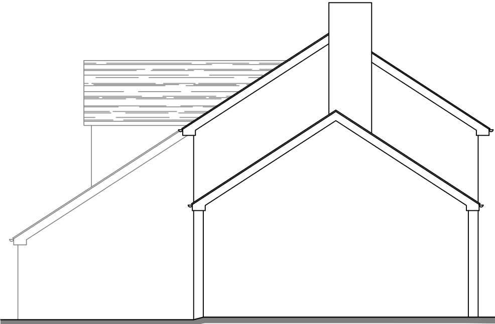
WEST ELEVATION
