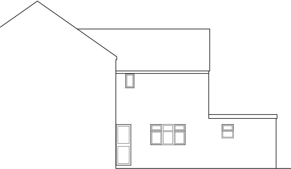
Side Elevation.
