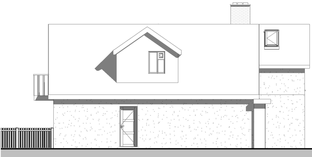
Proposed Elevation-Left side
