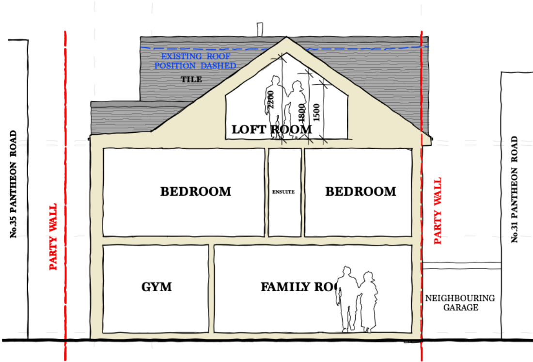
SHORT SECTION
