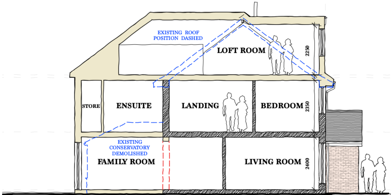
SHORT SECTION
