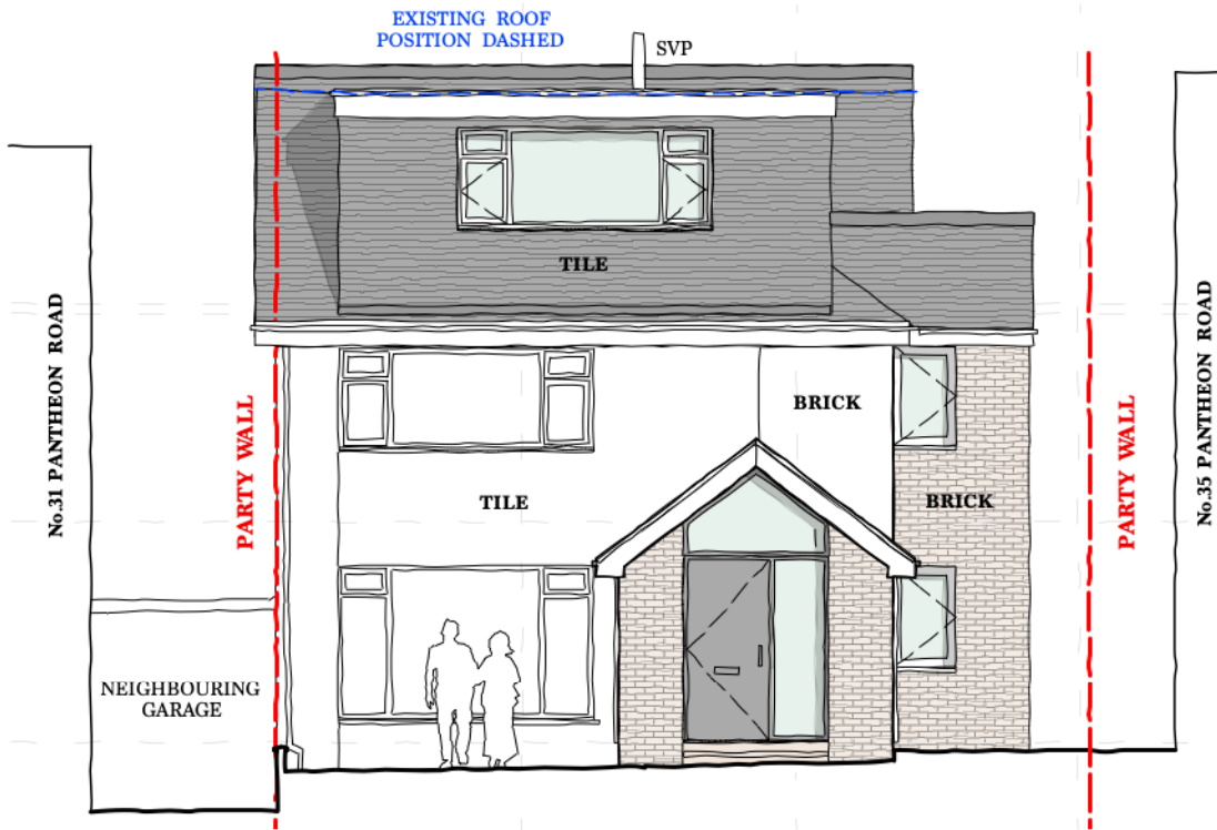
EAST ELEVATION
