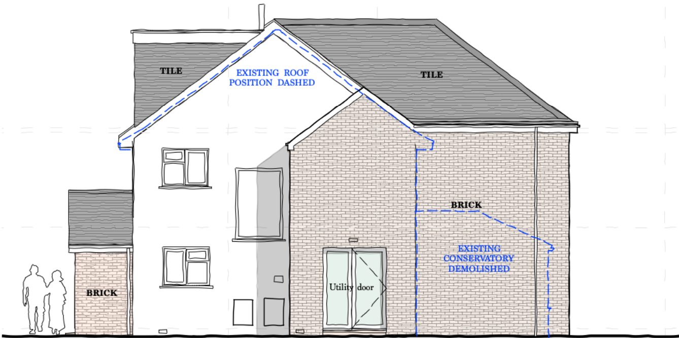
NORTH ELEVATION
