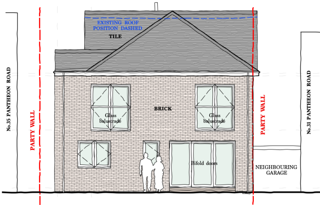
WEST ELEVATION
