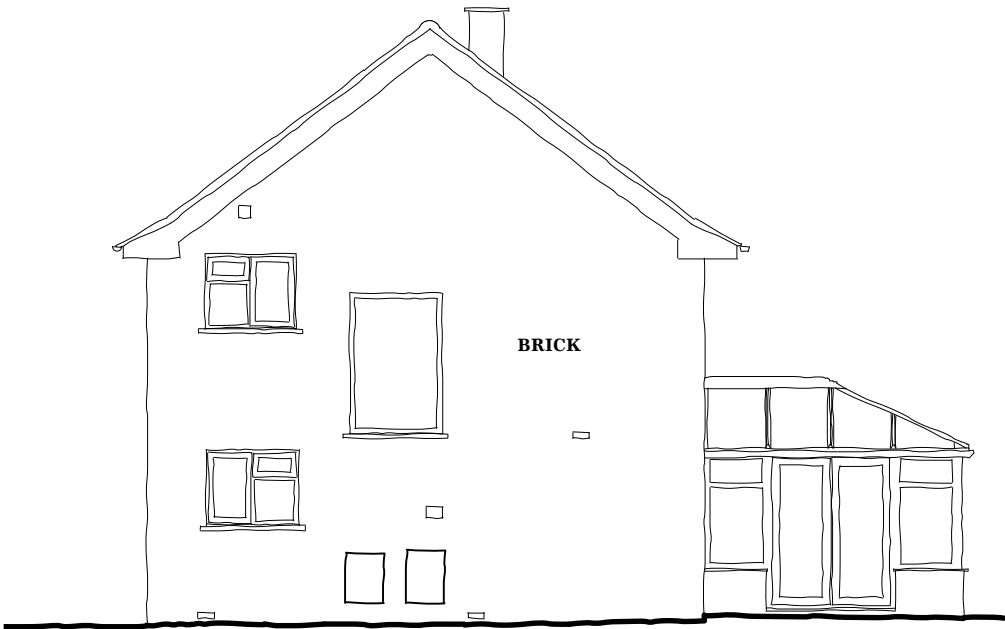
NORTH ELEVATION
