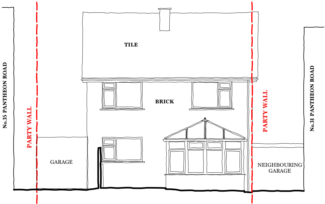
WEST ELEVATION
