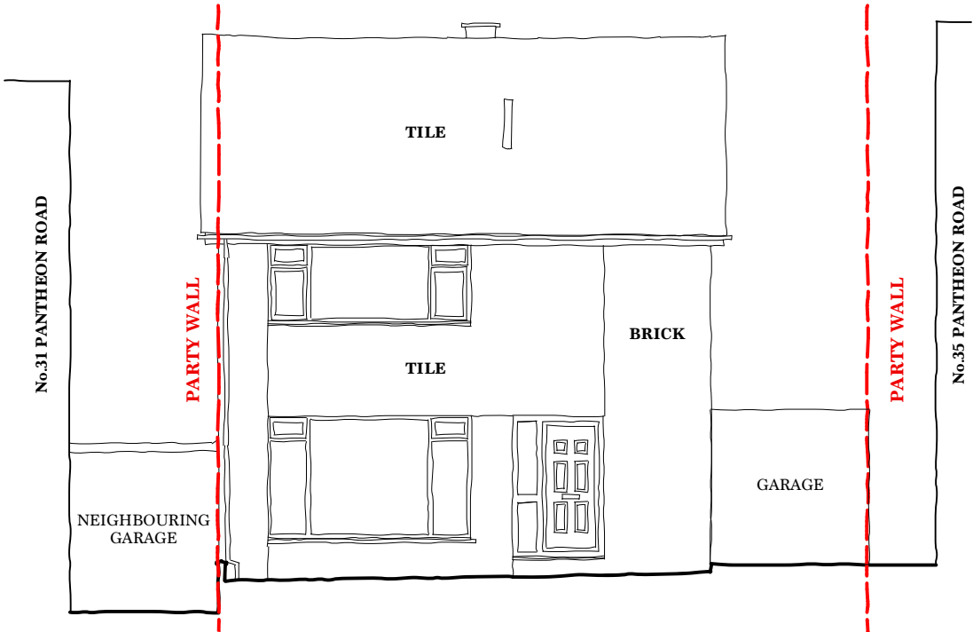
EAST ELEVATION
