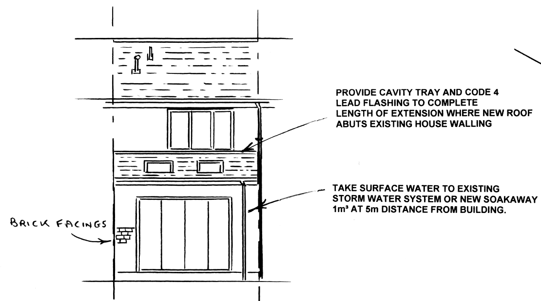
REAR ELEVATION (NORTH)
