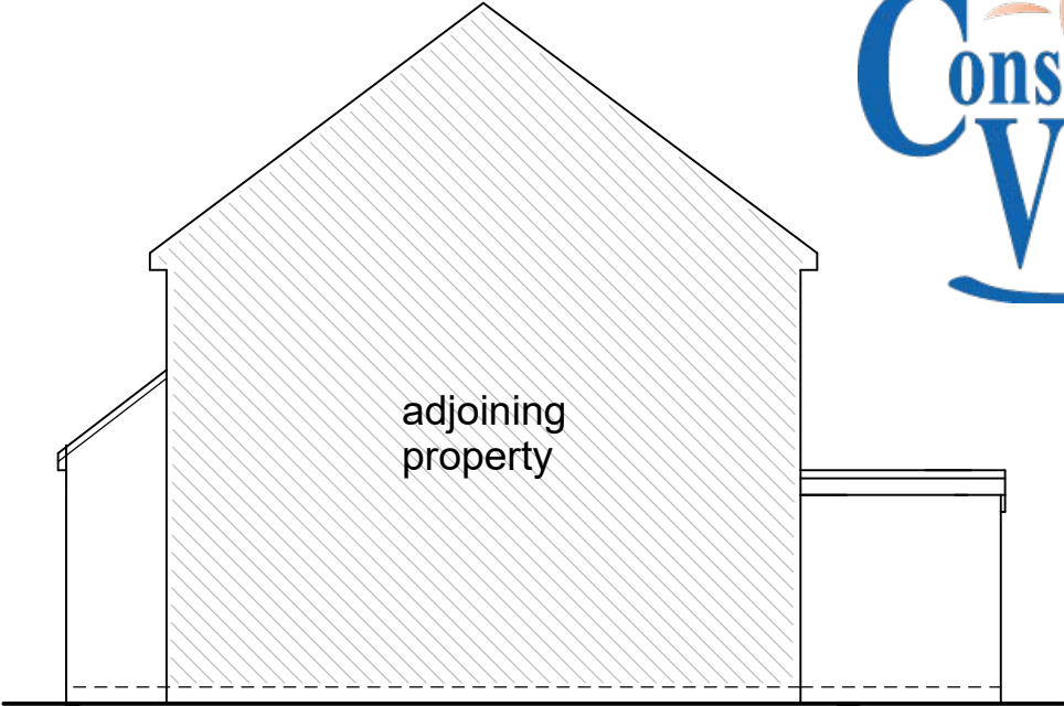
right (southwest) elevation
