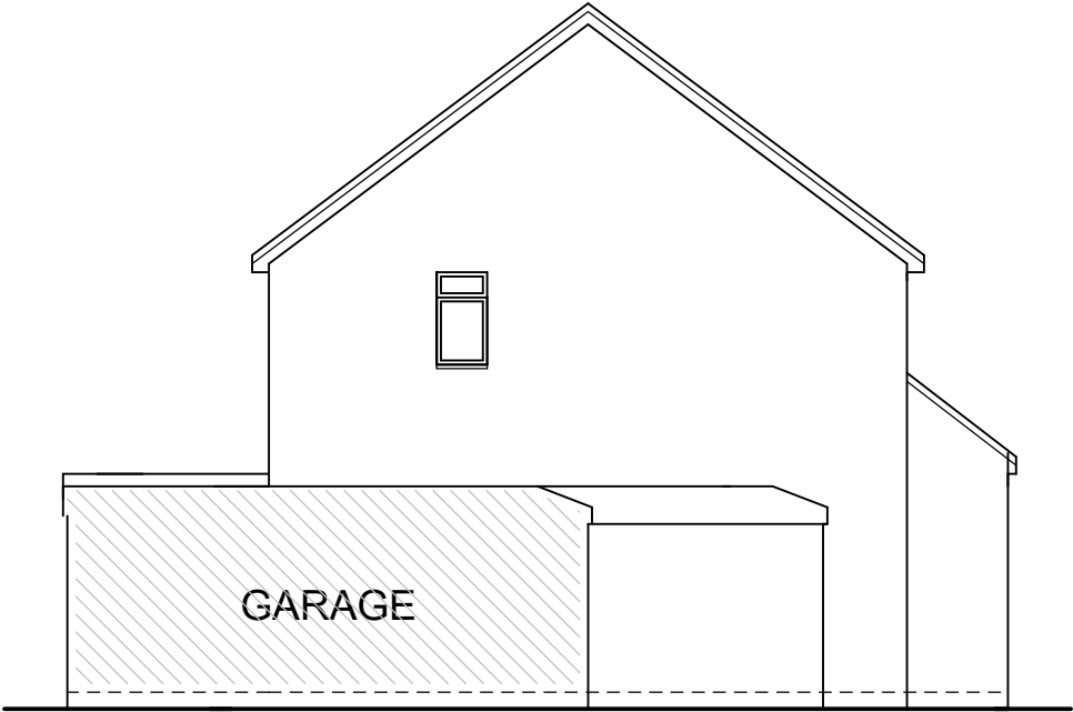
left (northeast) elevation
