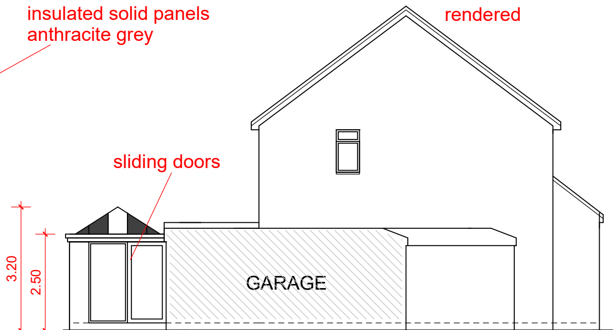
left (northeast) elevation
