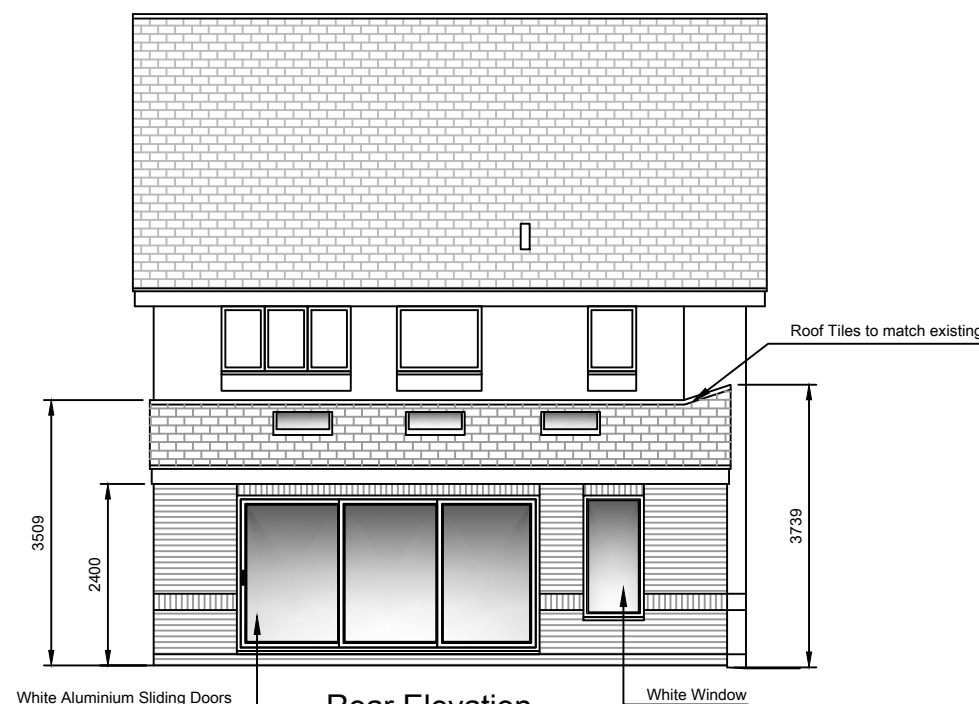
Rear Elevation
